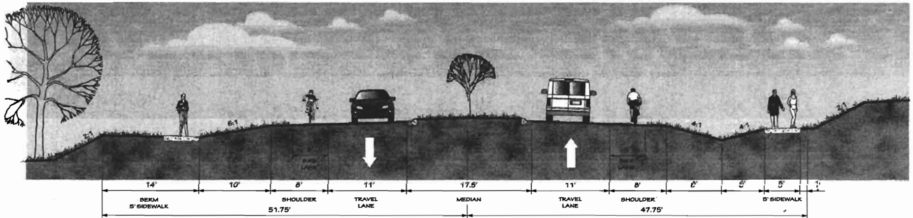
PROPOSED 2-LANE SHOULDER SECTION
